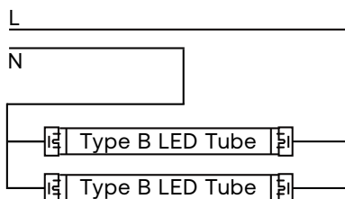
Shunted Sockets
