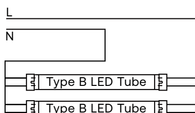
Unshunted Sockets
